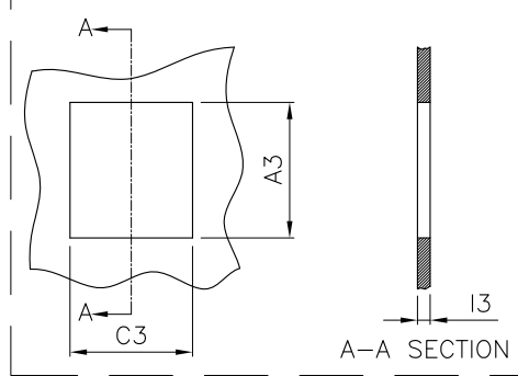
Figure D.2-Panel drawing
